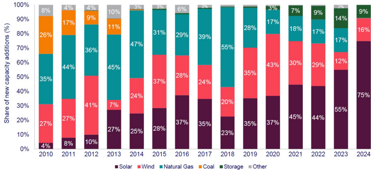
New U.S. electricity-generation capacity additions, 2010 – Q1 2024
